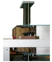
ROBA Duplex aggregate side view: 30 mm oscillation and pneumatic height adjustment to change sanding area
