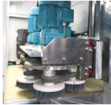
The Profi Disc as optional aggregate at machine inlet or outrun
