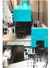
Transverse cleaning unit, optional also from bottom.
